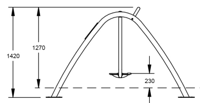
SIDE ELEVATION
